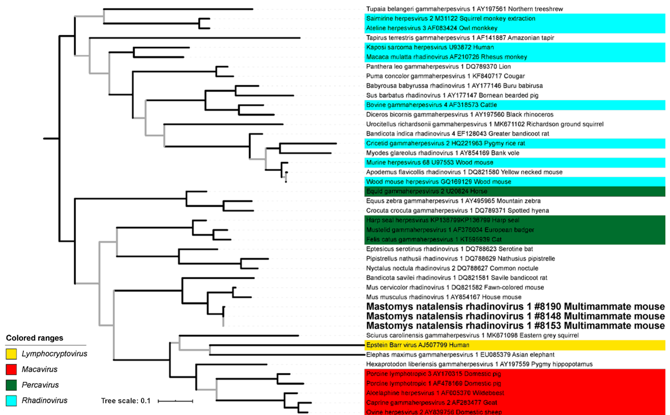
Fig. 3 Maximum-likelihood tree of gammaherpesviruses based on blocks of conserved amino acids in glycoprotein B. For explanation see legend of Fig. 2
